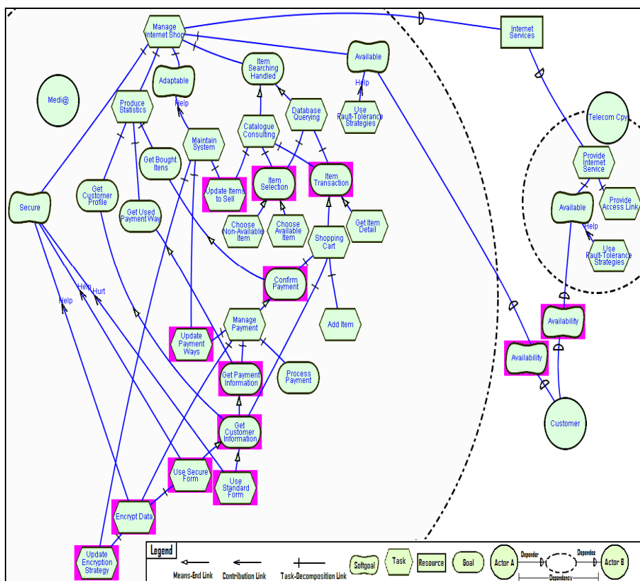
Fig. 1. The Medi@ Strategic Rationale Model
