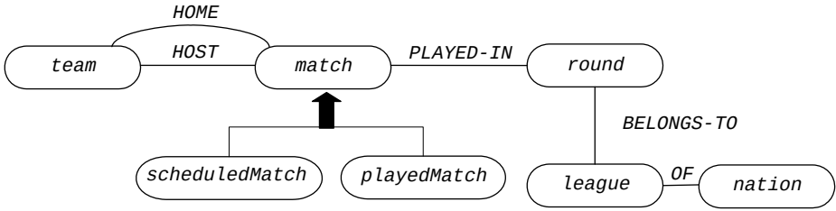
Fig. 2. Diagrammatic representation of the football leagues example
