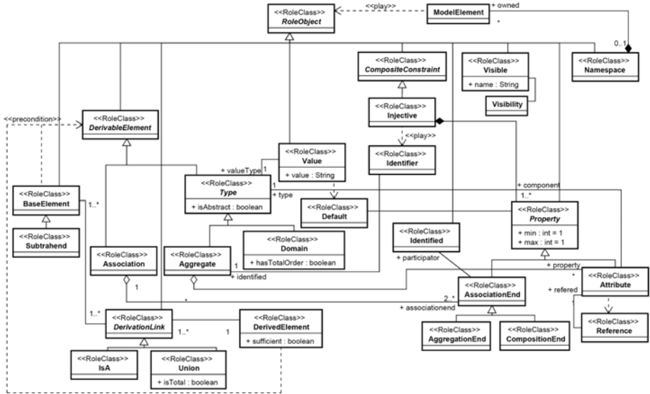
Fig. 5. Subset of the GeRoMe meta model
