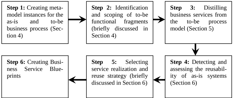
Fig. 2. GAMBUSE steps
