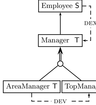
Fig. 4. Transitions employee-to-manager and area-to-top manager
