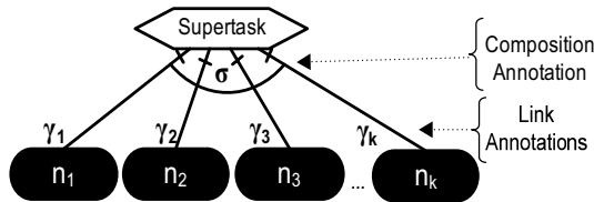
Fig. 3. Composition and link annotations
