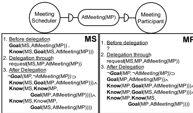
Fig. 7. A motivating example
