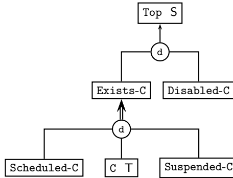
Fig. 3. Status classes
