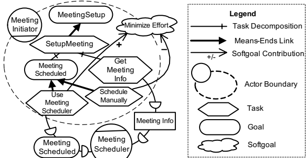
Fig. 2. SR model for the meeting initiator
