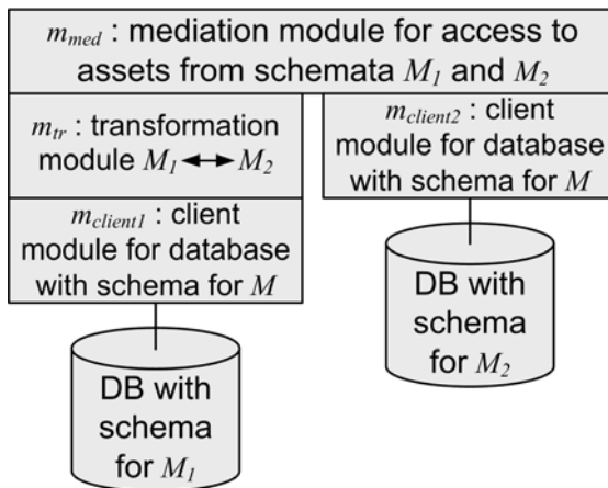
Fig. 10. A sample module organisation
