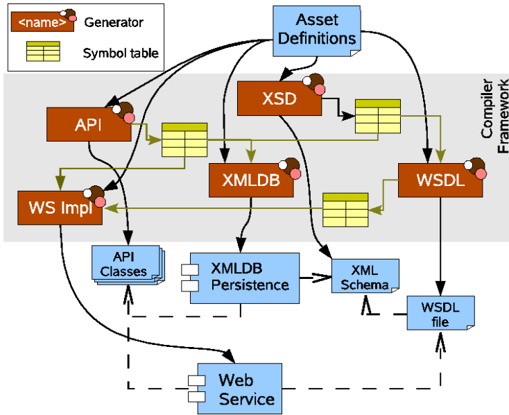
Fig. 11. Compiler framework
