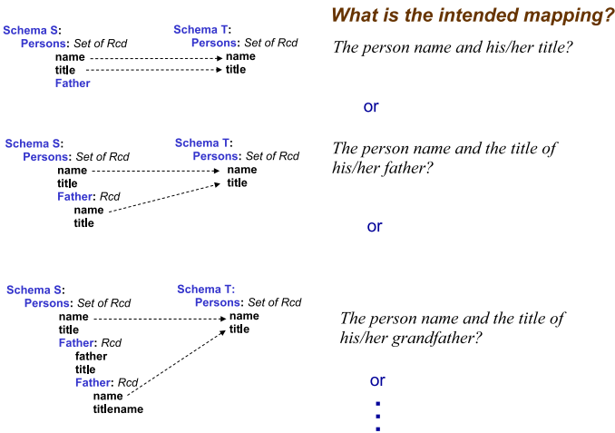
Fig. 12. Unlimited candidate mappings due to recursive types
