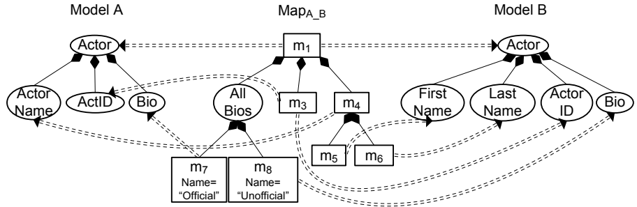
Fig. 3. A more complicated mapping between the models in Figure 1; Map_{A,B} contains an element that does not appear in either A or B
